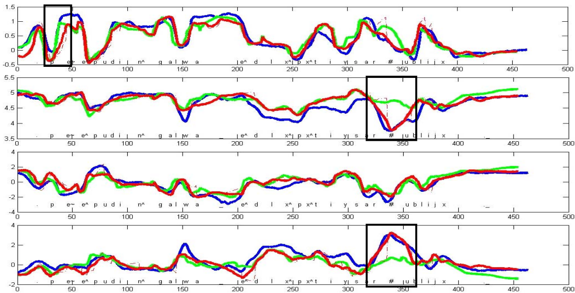
Figure 3. Comparing trajectory formation systems (blue: natural reference; red: concatenation/selection TDA; green: contextual phoneme-HMM) with a natural test stimulus (blue). From top to bottom: geometric parameters: lip aperture, width and protrusion; articulatory parameters: jaw aperture, lips rounding/spreading. Major discrepancies between TDA and contextual phoneme-HMM are enlighten
