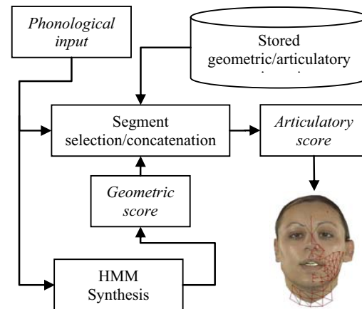
Figure 1. The proposed trajectory formation system TDA.
